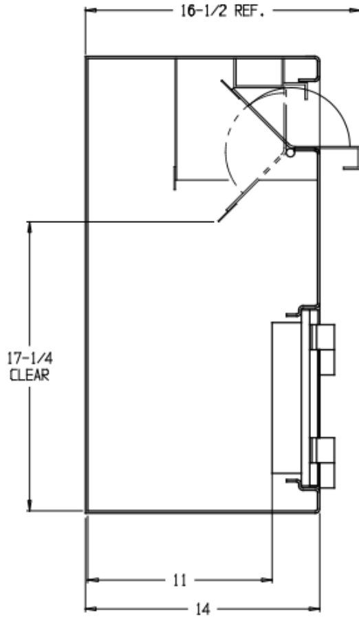
SECTION VIEW
