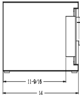
SECTION VIEW
